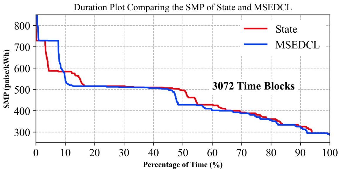
Figure 39. Duration plot of State SMP and MSEDCL
