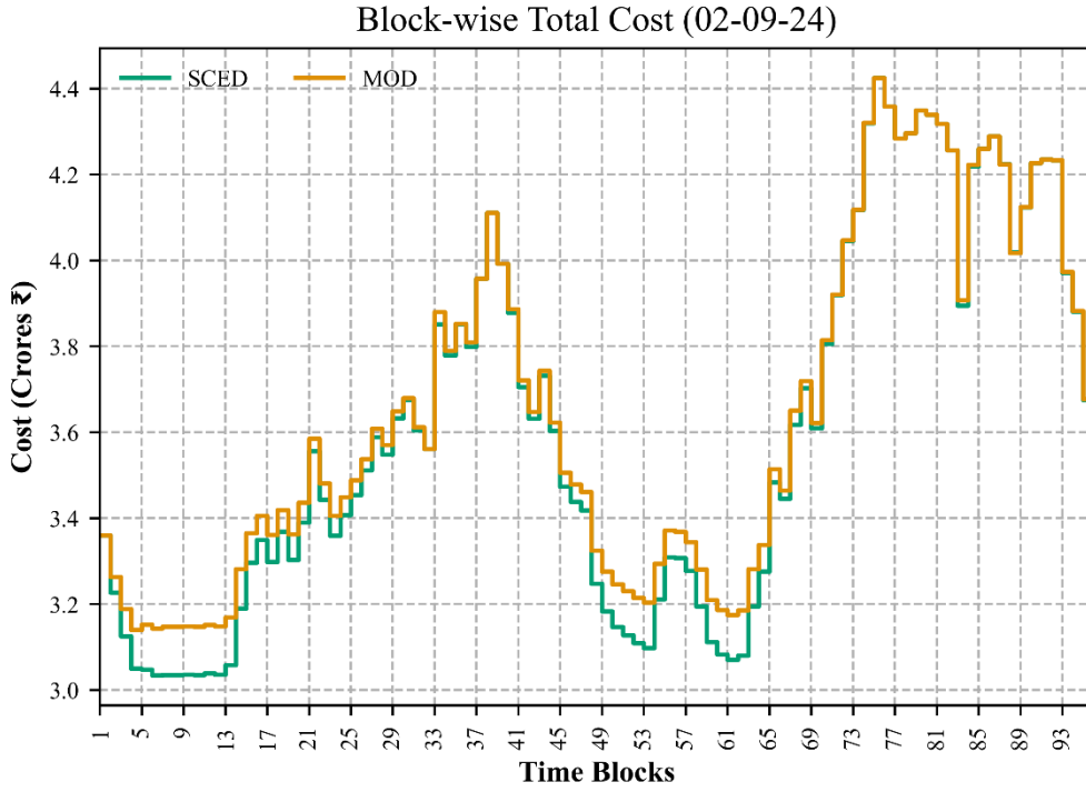
Figure 8. Diurnal plot of block wise cost for a single day
