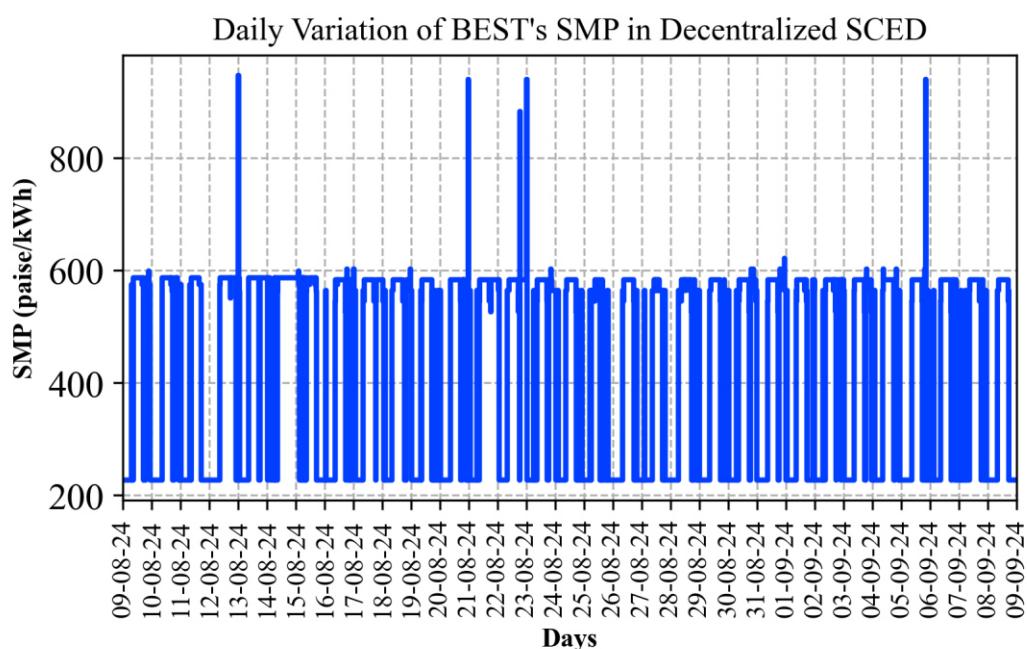
Figure 36. Diurnal variation of the BEST's SMP
