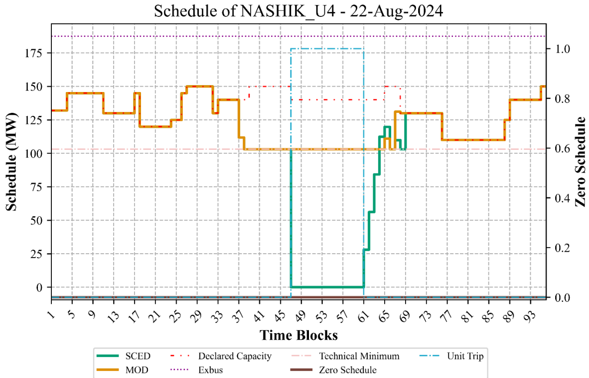
Figure 55. Schedule of the NASHIK_U4 unit experiencing trip.
