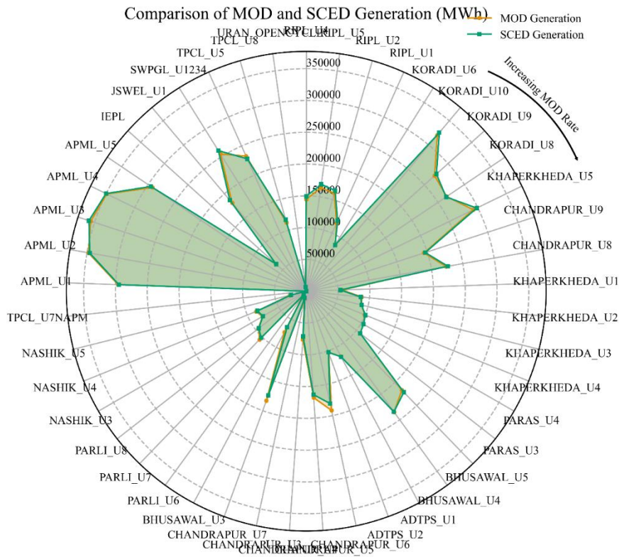
Figure 17. Plant wise total generation comparison
