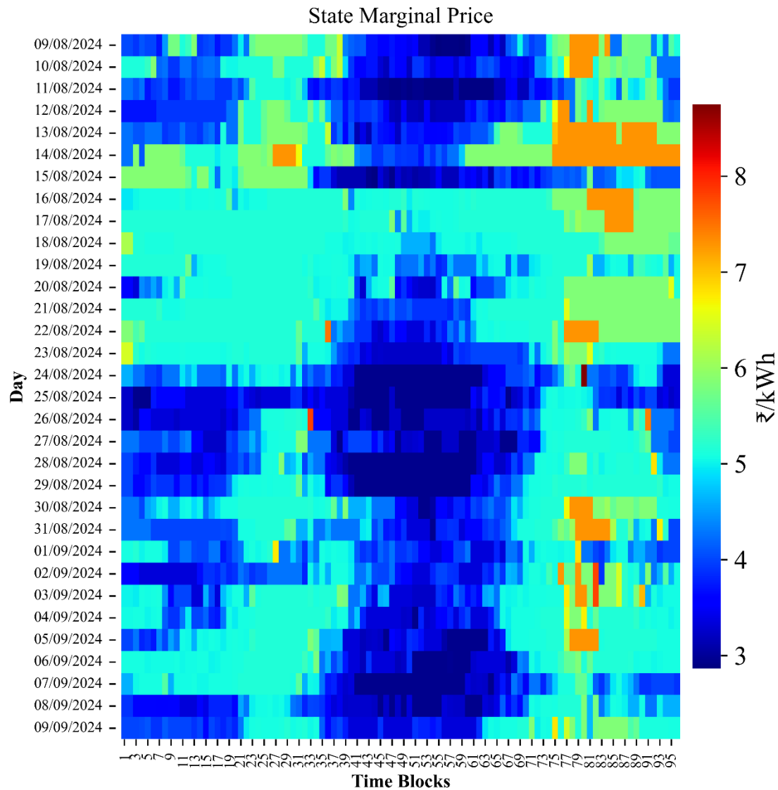
Figure 43. SMP variation in centralized SCED
