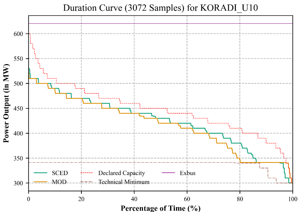
Figure 26. Duration plot of power output for Koradi
