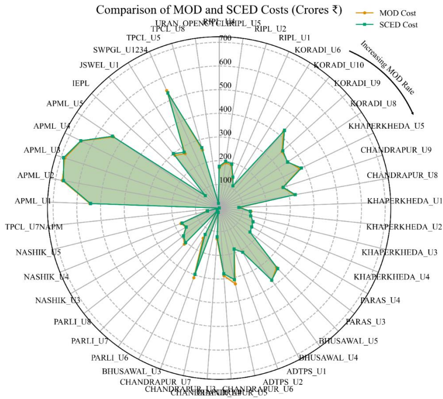
Figure 18. Unit wise total cost comparison
