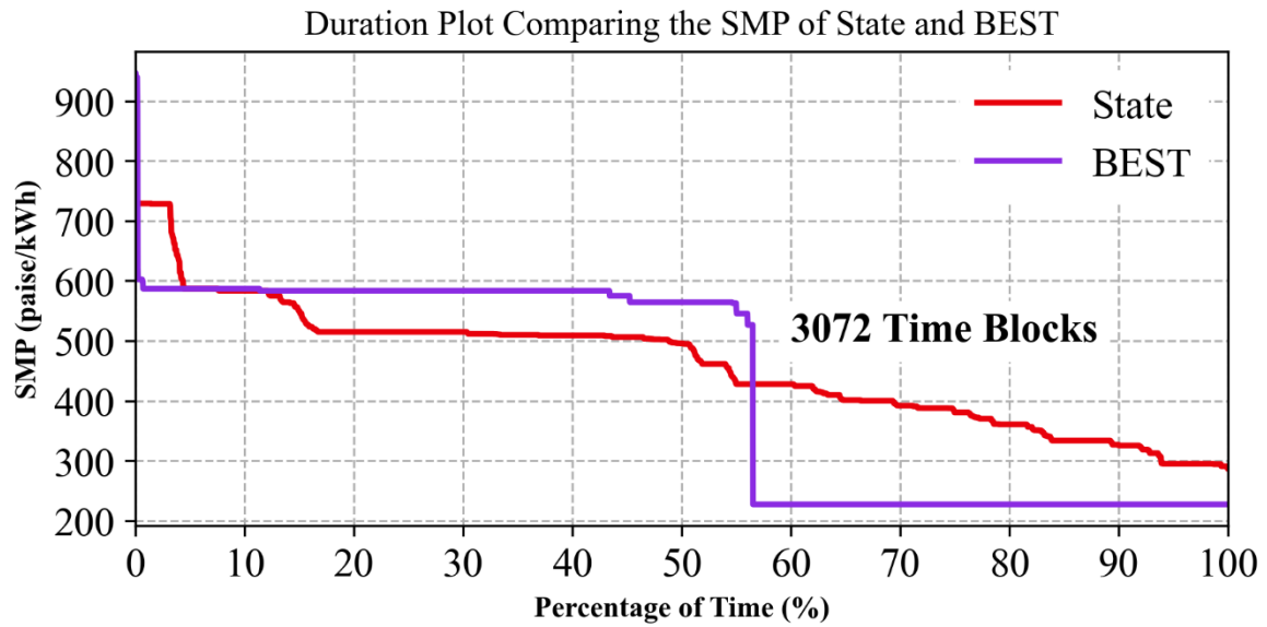
Figure 40. Duration plot of State SMP and BEST
