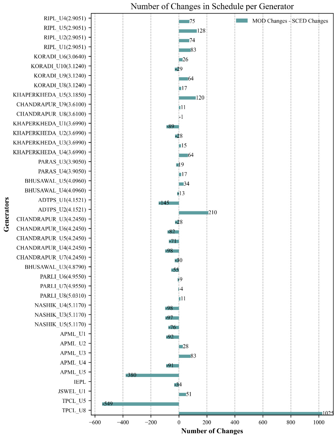
Figure 25. Generator-wise difference in perturbations in MOD and SCED.
