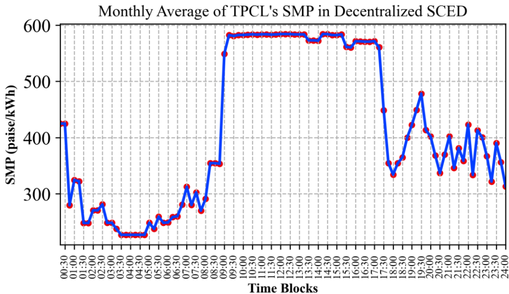
Figure 35. Diurnal variation of the TPCL's SMP
