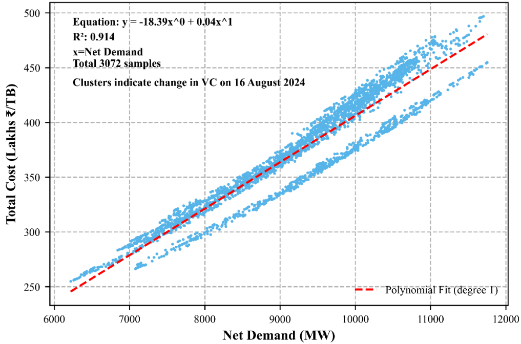
Figure 15. Scatter plot between total cost and Demand met.
