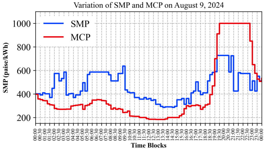
Figure 44. Diurnal variation of SMP and MCP
