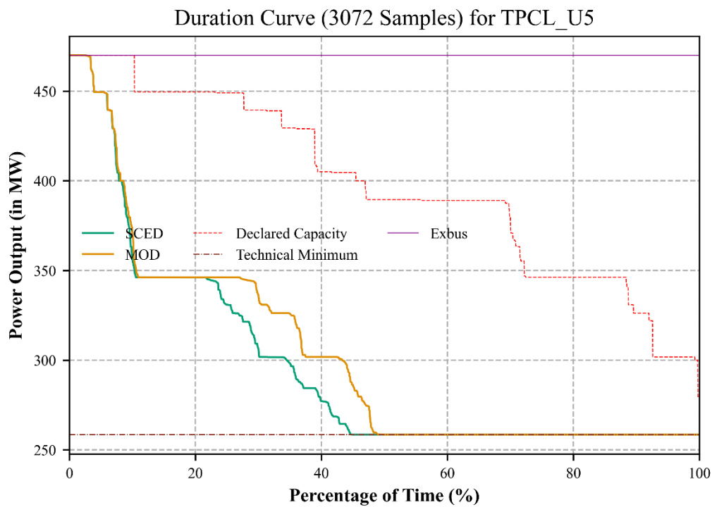
Figure 27. Duration curve of TPCL U5.
