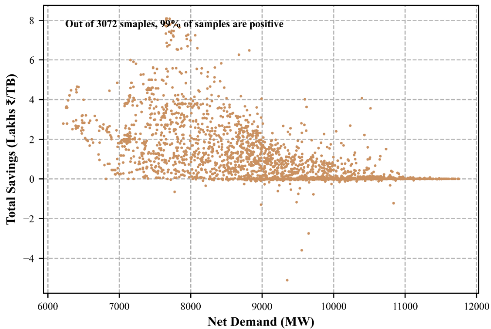
Figure 16. Scatter plot between saving and demand
