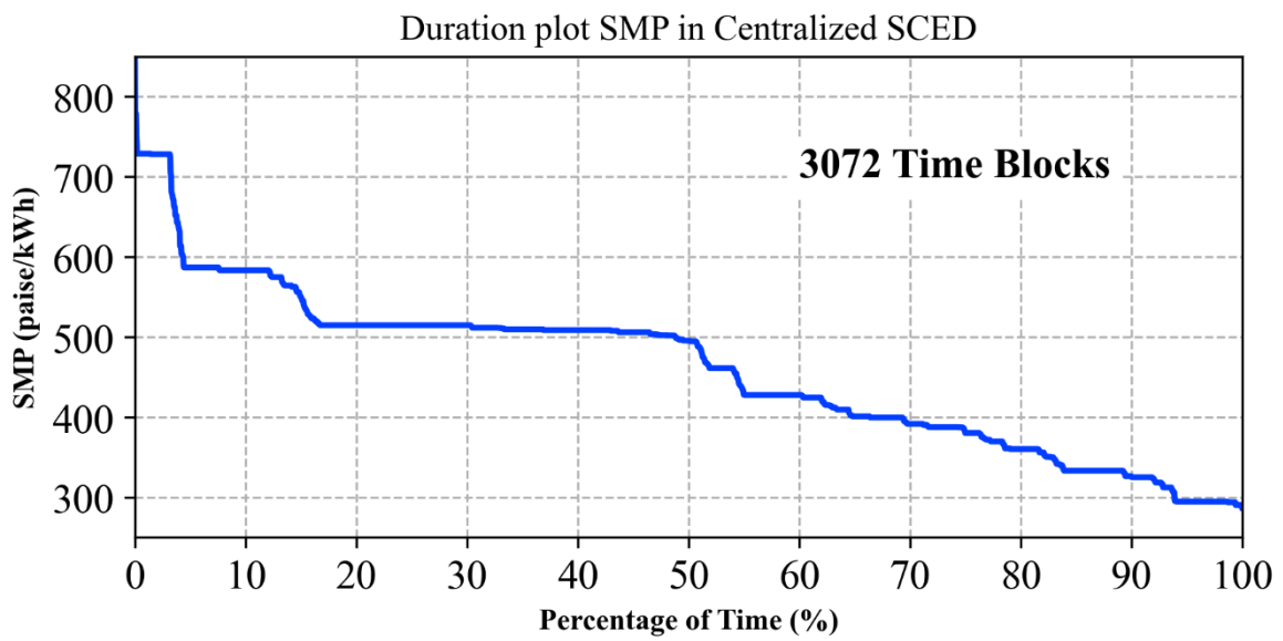
Figure 29. Duration plot of SMP.
