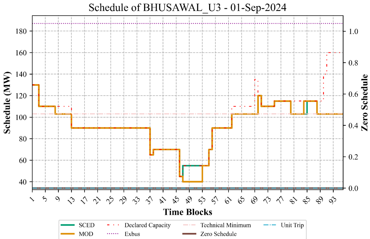
Figure 54. Schedule of BHUSAWAL_U3 operating below adjusted Tech. minimum.
