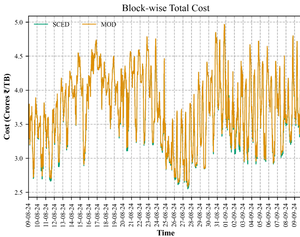
Figure 7. Block wise total cost of MOD and SCED
