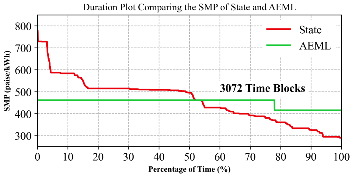
Figure 42. Duration plot of State SMP and AEML
