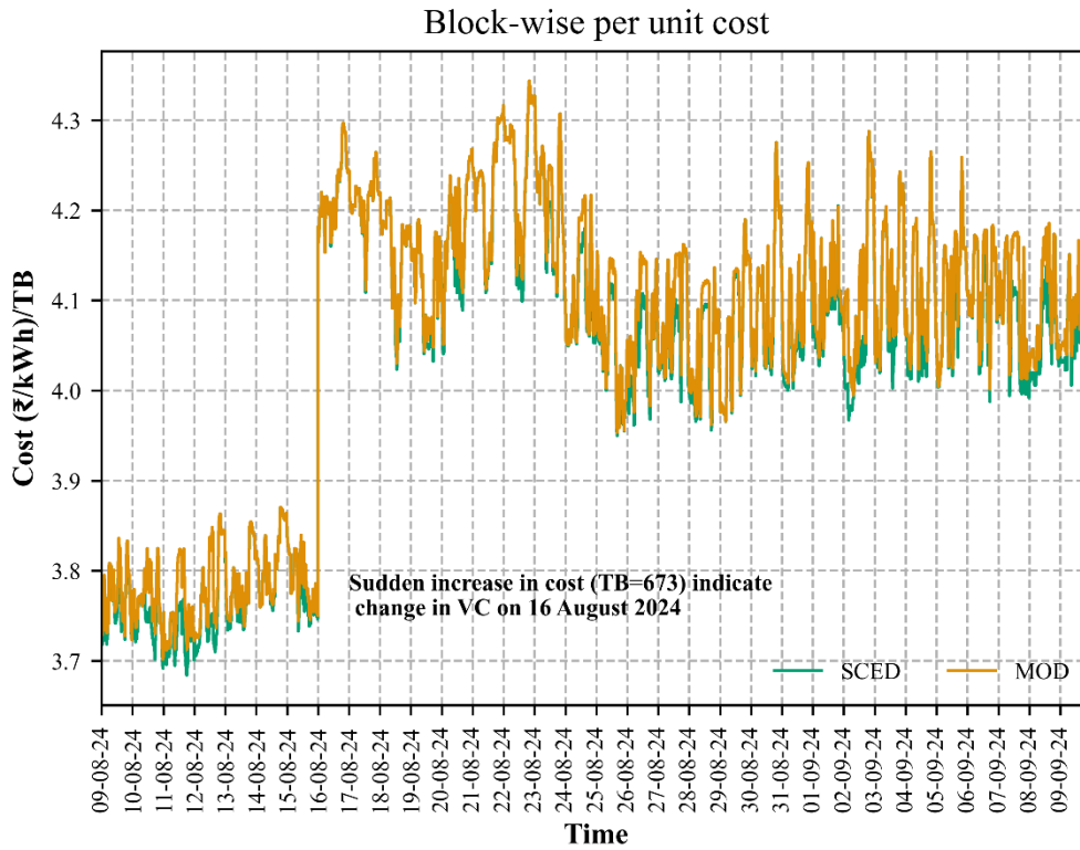
Figure 11. Block wise per unit total cost.
