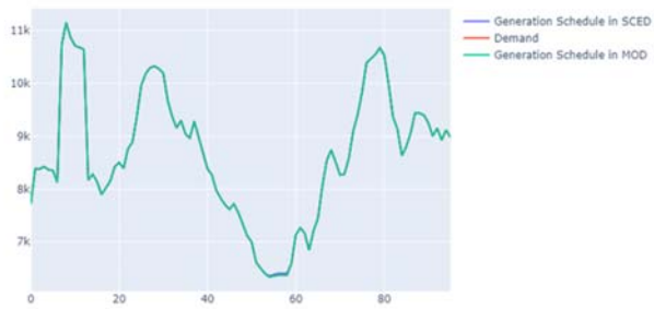
Demand VS Scheduled Power (MSDCL)
