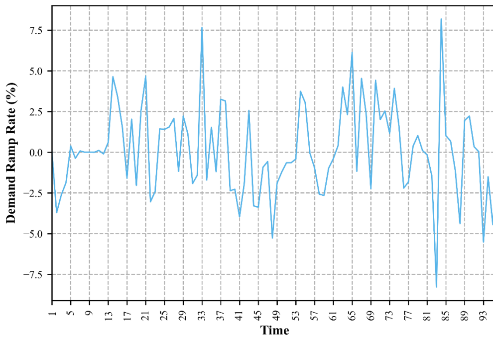
Figure 6. Variation in demand ramp on a sample day (02-09-24)
