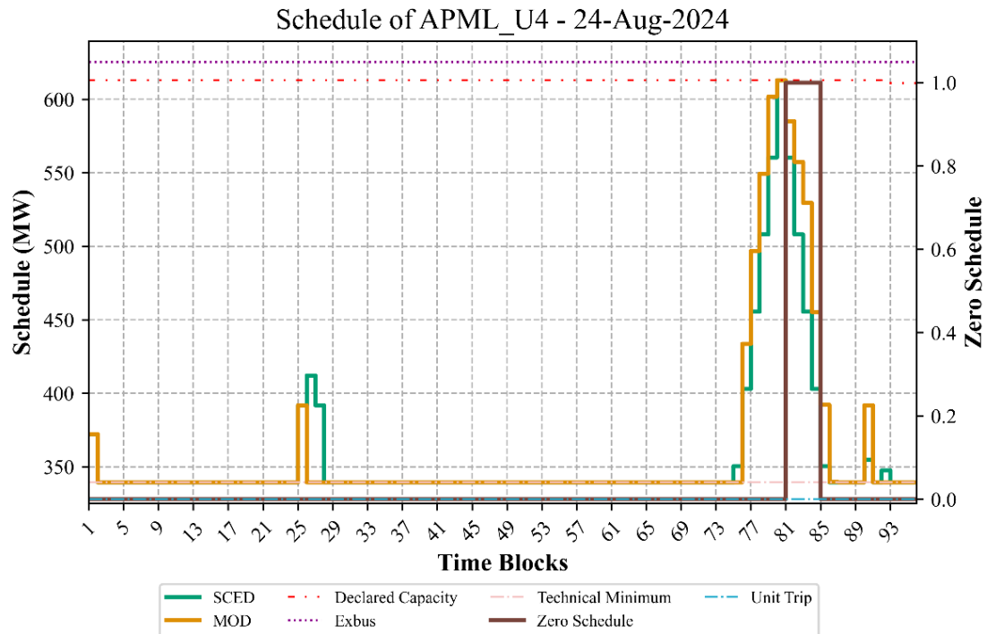
Figure 53. Inconsistent declared capacity with zero schedule
