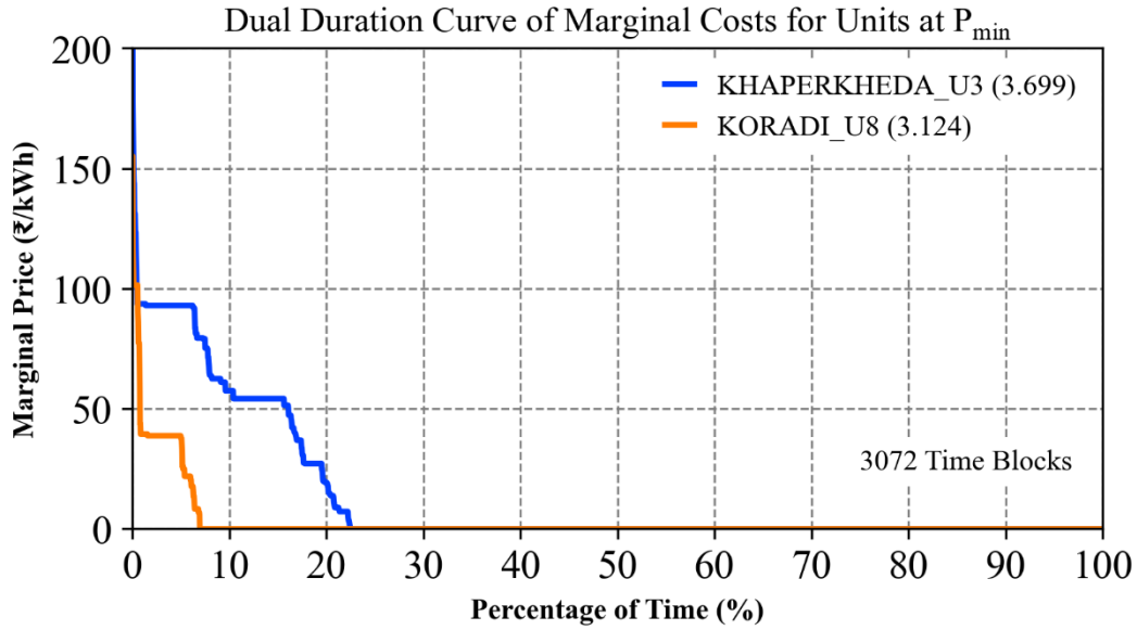
Figure 52. Duration curve of the marginal cost for units, relatively cheaper, operating at P_{min}
