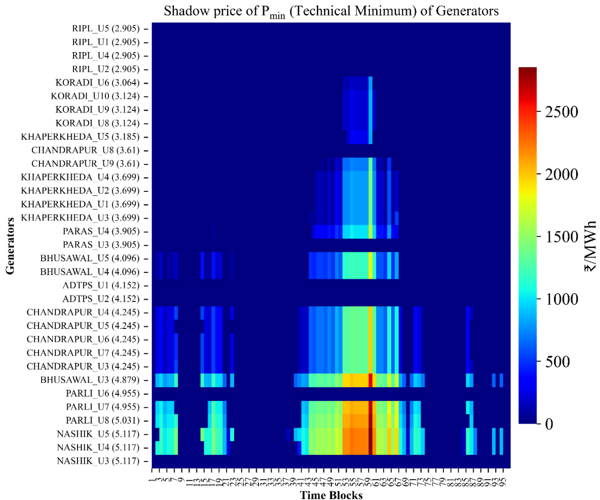
Figure 50: Heat map for marginals of technical minimum
