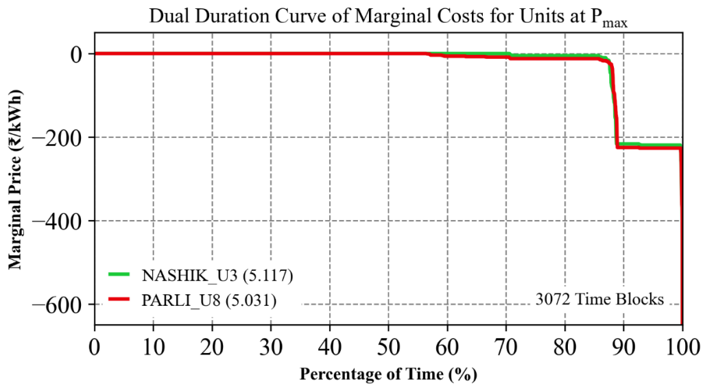
Figure 48. Duration curve of the marginal cost for units, relatively expensive, operating P_{max}
