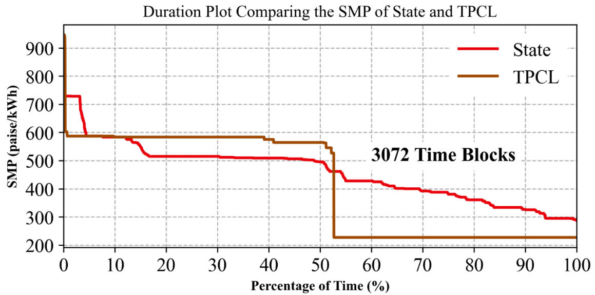
Figure 41. Duration plot of State SMP and TPCL
