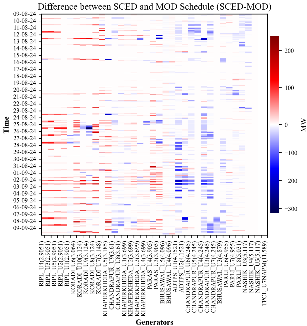
Figure 21. Difference between SCED and MOD schedule.
