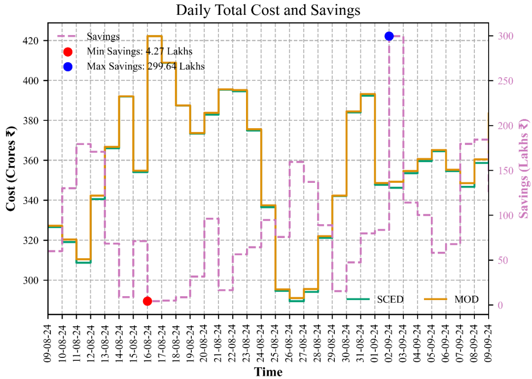
Figure 10. Daily cost savings
