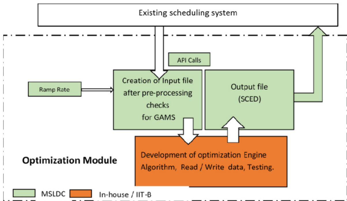
Figure 3. Proposed system implementation
