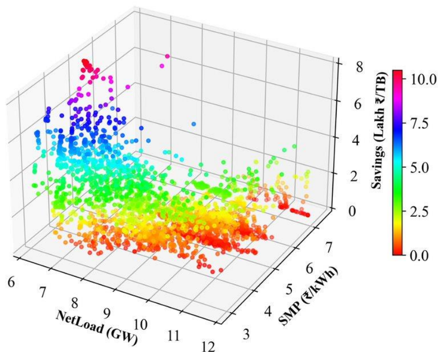
Figure 32. Correlation between savings, netload and SMP
