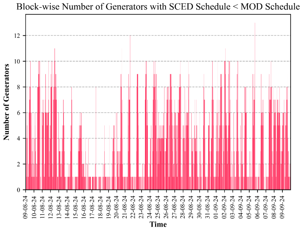
Figure 24. Block-wise no. of generators when SCED schedule < MOD schedule.
