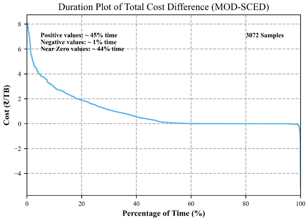
Figure 14. Duration plot of cost difference.
