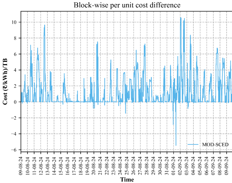
Figure 9. Block wise per unit cost difference of MOD and SCED
