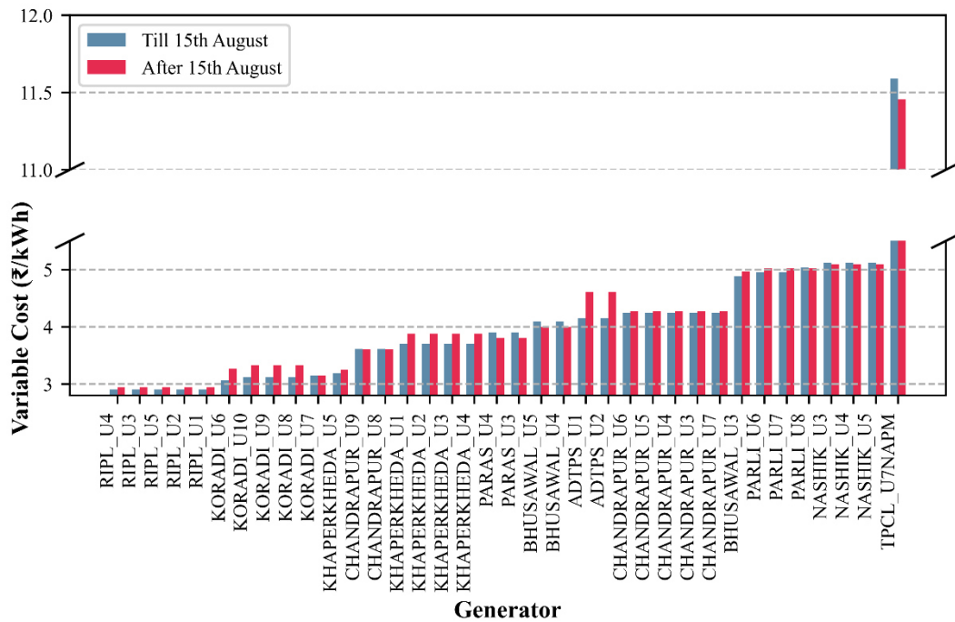
Figure 13. Variable cost in ascending order
