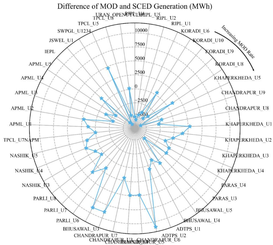
Figure 19. Energy generation difference in MOD and SCED
