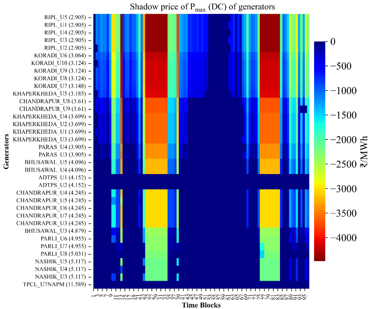
Figure 47. Heat map for marginals of declared capacity.
