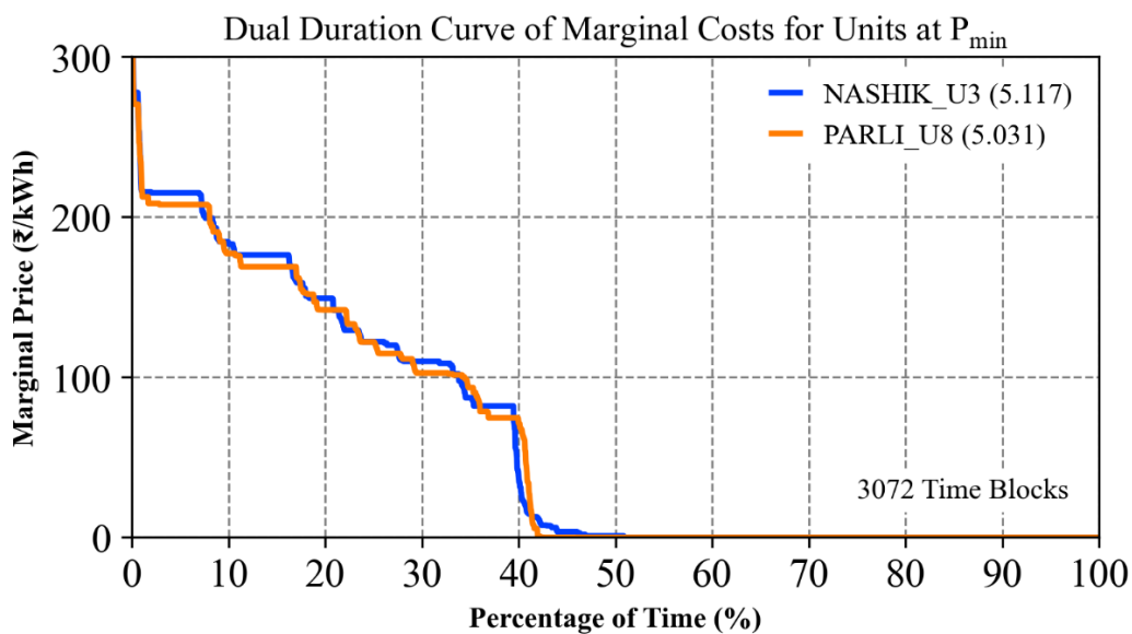
Figure 51. Duration curve of the marginal cost for units, relatively expensive, operating at P_{min}
