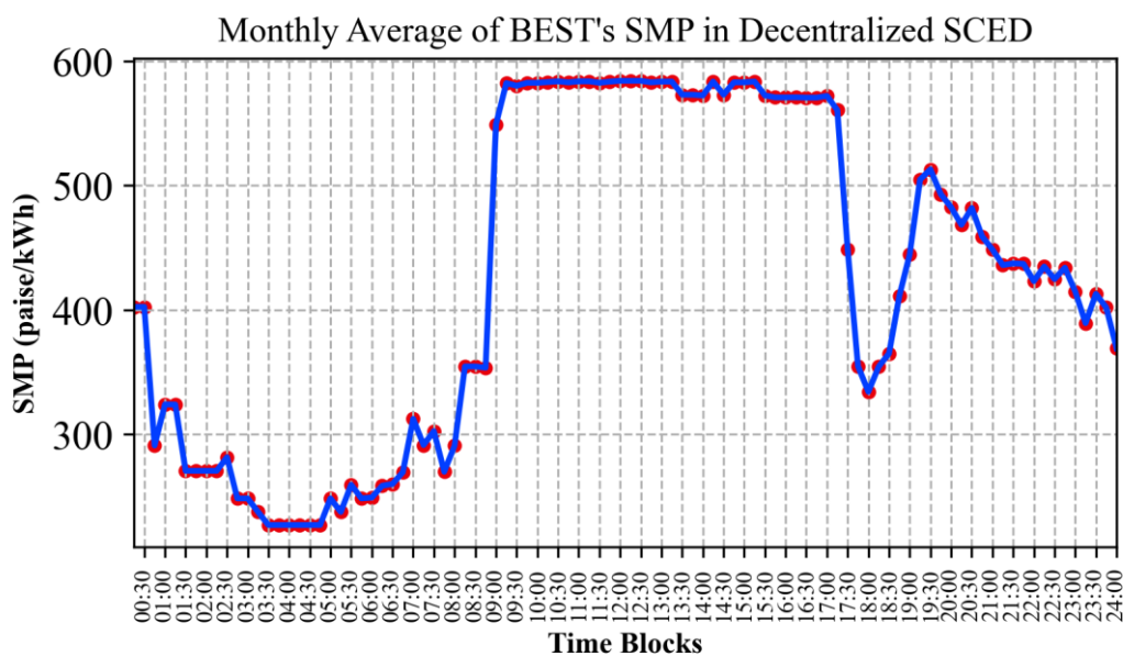
Figure 37. Discom SMP for BEST
