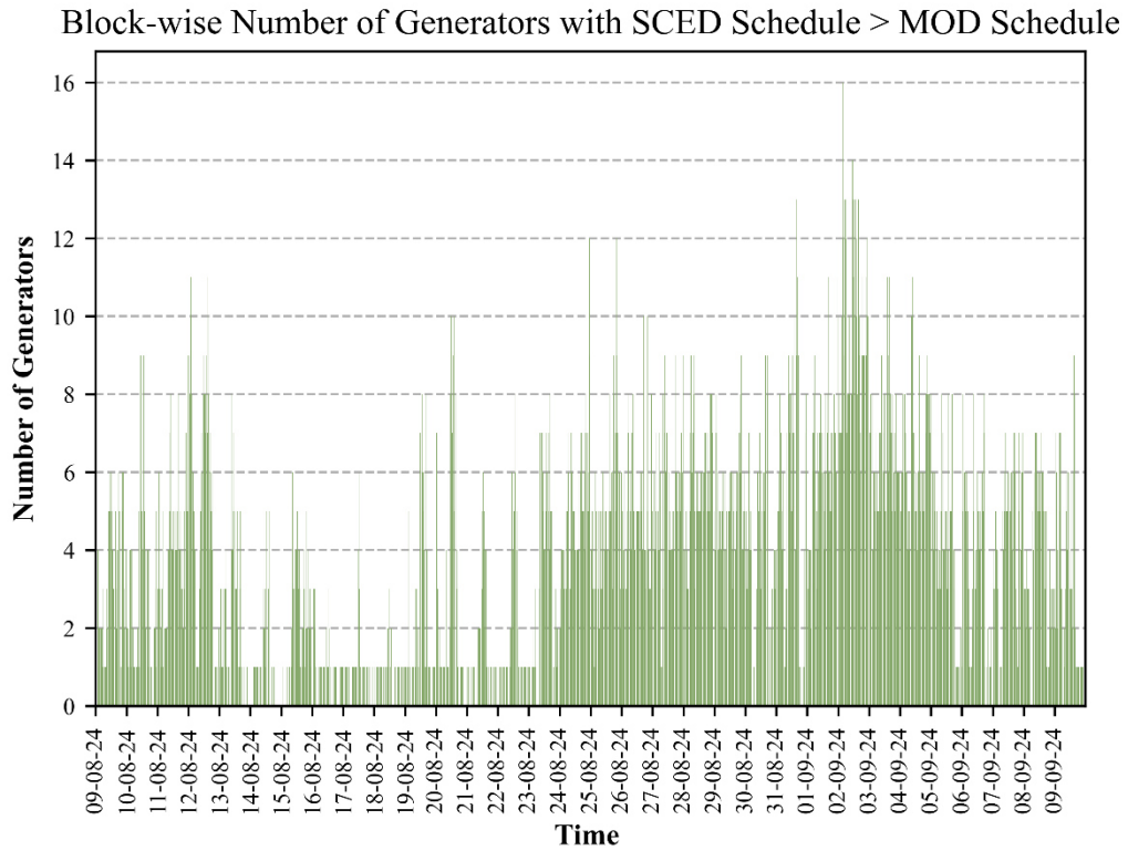
Figure 23. Block-wise no. of generators when SCED schedule > MOD schedule.
