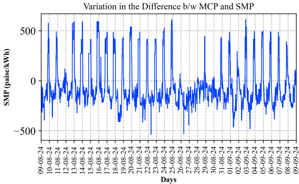
Figure 46: Diurnal plot of variation of Diff between MCP and SMP
