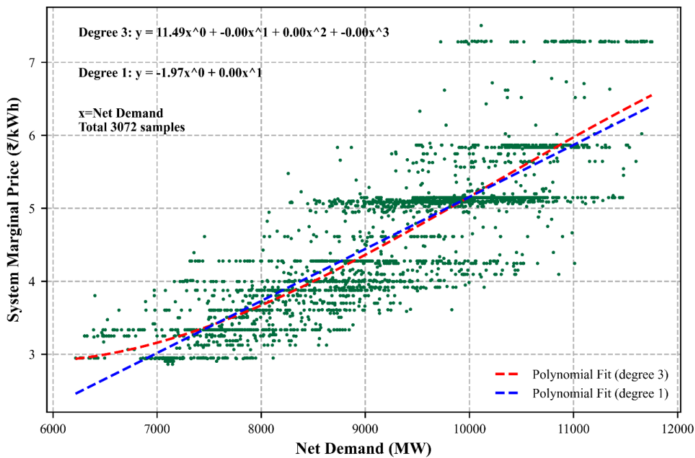
Figure 31. Correlation of SMP with net demand.
