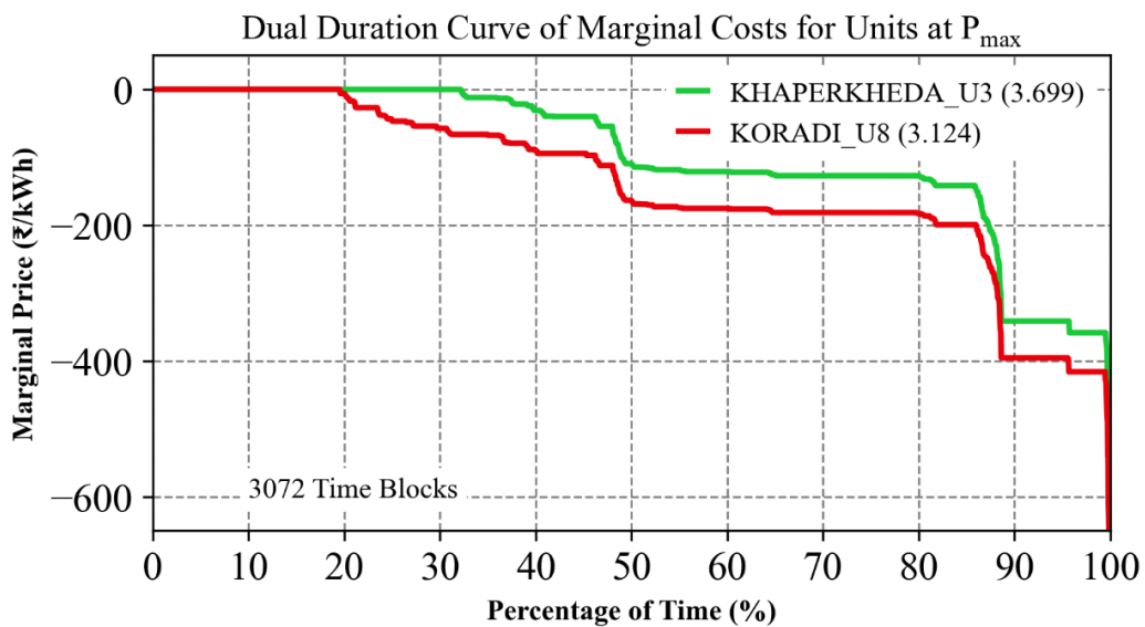
Figure 49. Duration curve of the marginal cost for units, relatively cheaper, operating P_{max}
