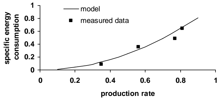
Figure 1. Variation in specific energy with production rate
